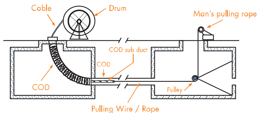
<Man's Pulling system>
