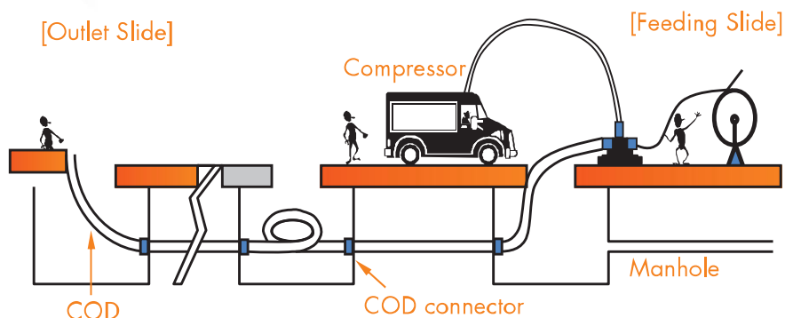
<Air Blowing system>
